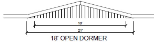
FLAT & VAULTED 23'-4" WIDES AND BIGGER
